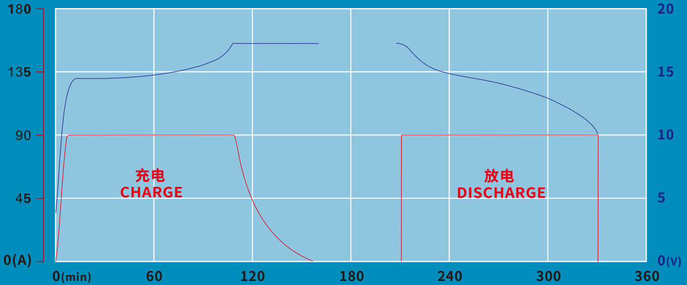
▲ TSWB-LP12V90AH在25°C环境下90A充放电特性 TSWB-LP12V90AH CHARGE AND DISCHARGE BY 90A AT TEMPERATURE OF 25°C
